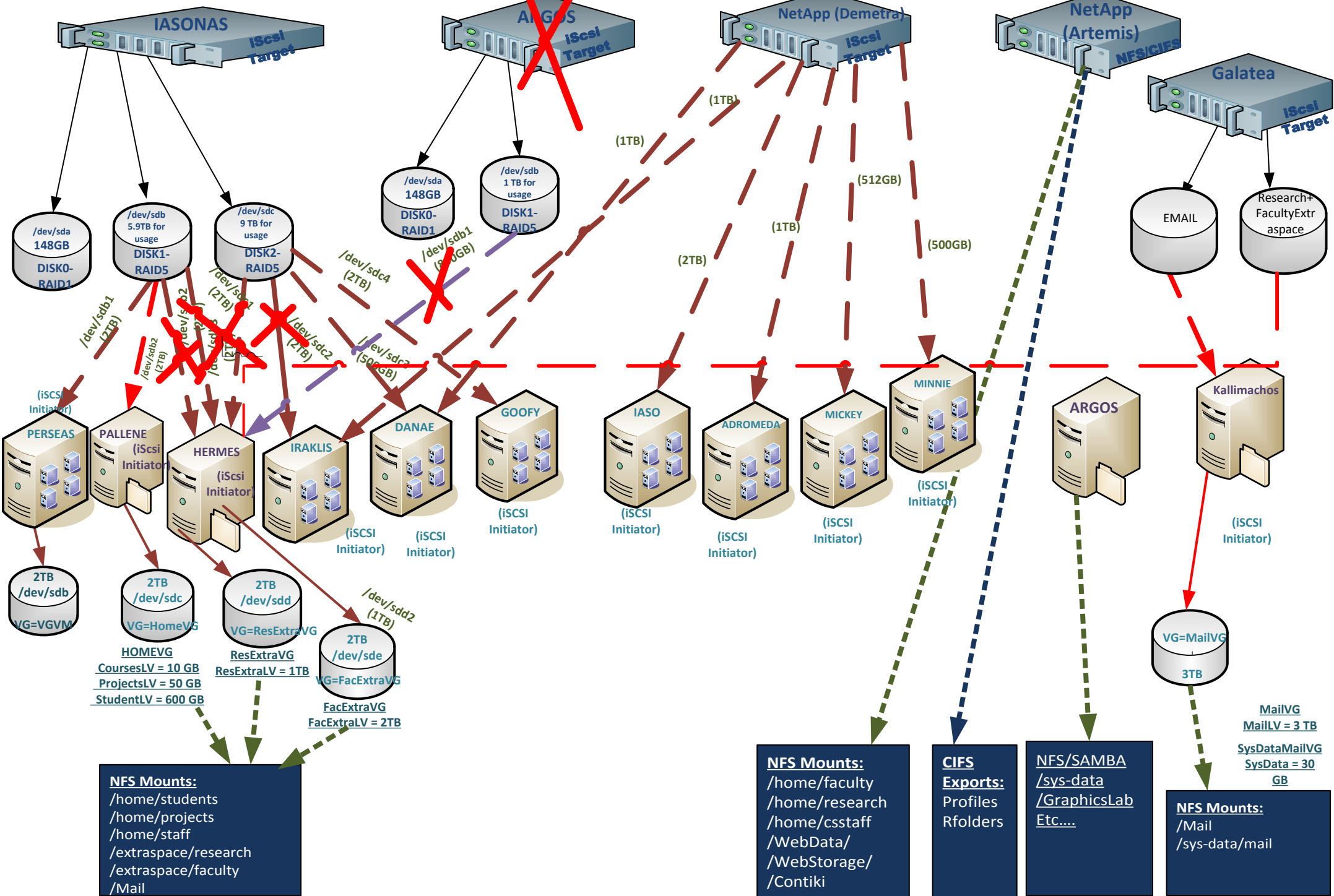
Disk Space Allocation Diagram for iScsi and NFS, CIFS Storage
